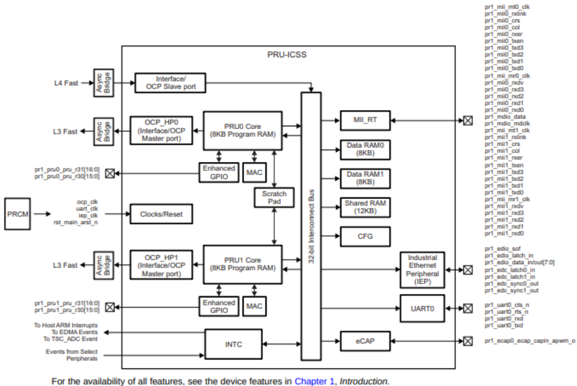
Figure 4-2. PRU-ICSS Integration
