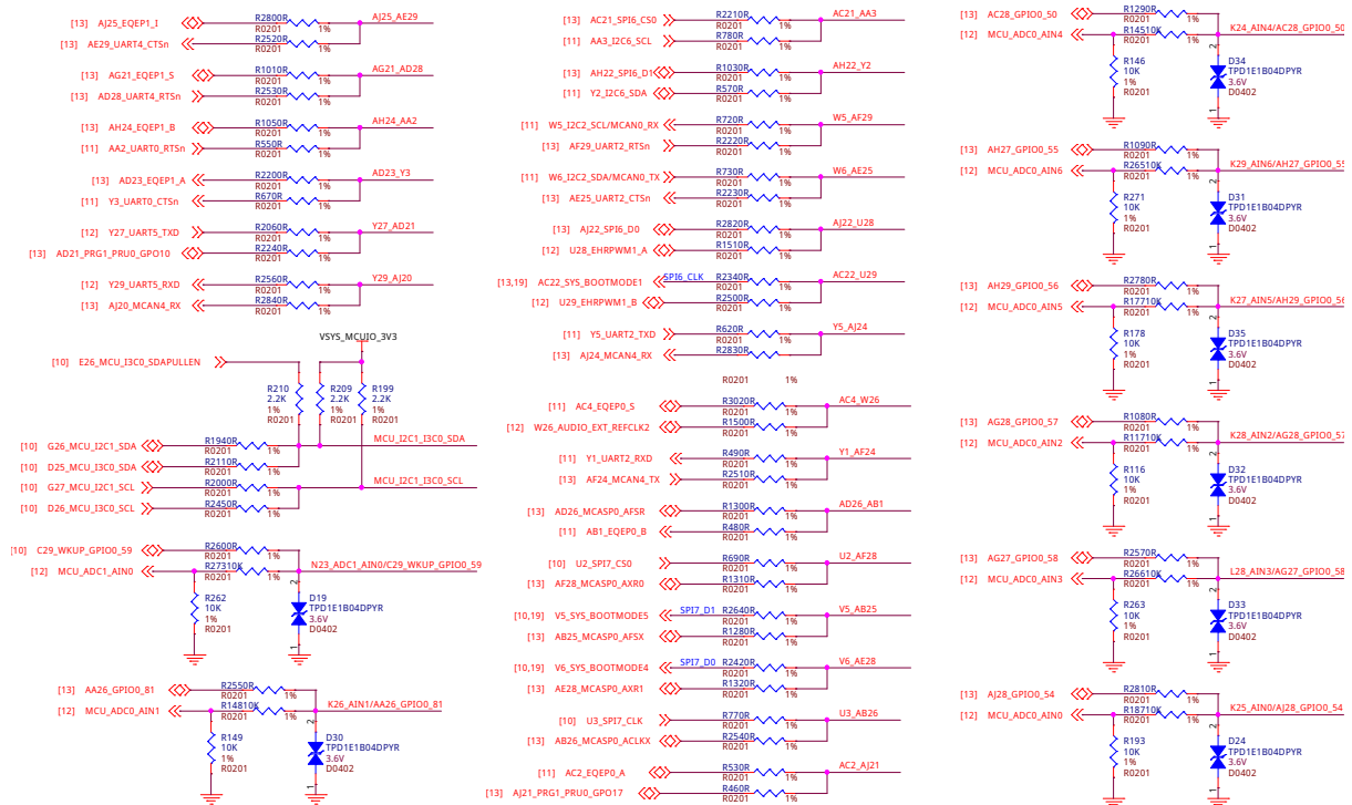
Fig. 3.22: P8 &amp; P9 cape header pins that uses two pins of SoC
